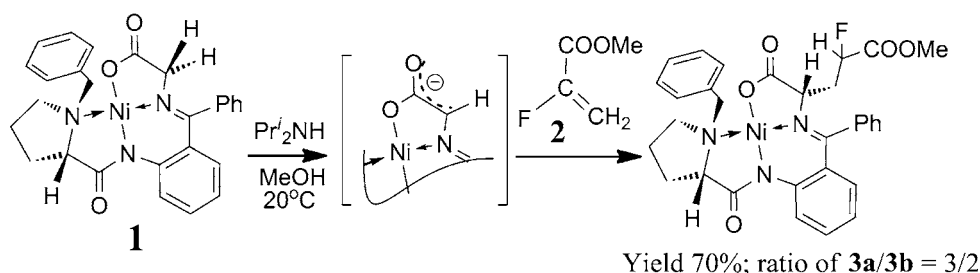
Scheme 1 Key step in the asymmetric synthesis of FGlu
